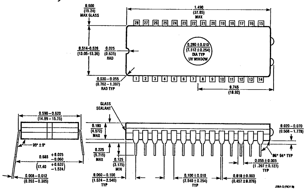
28 Lead EPROM Dual In-Line Cerdip Package (JQ) Small Window Order Number 27CP128Q350/883, 27CP128Q300/883 or 27CP128Q250/883 NS Package Number J28AQ
